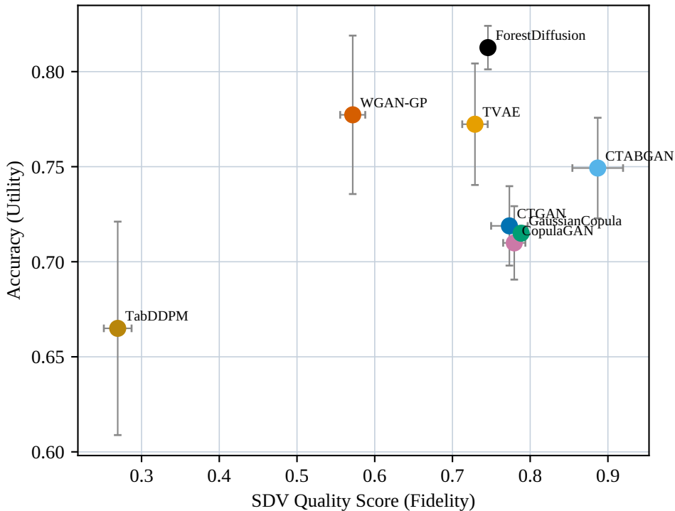
Adult: SDV Quality Score (Fidelity) vs Accuracy (Utility)
